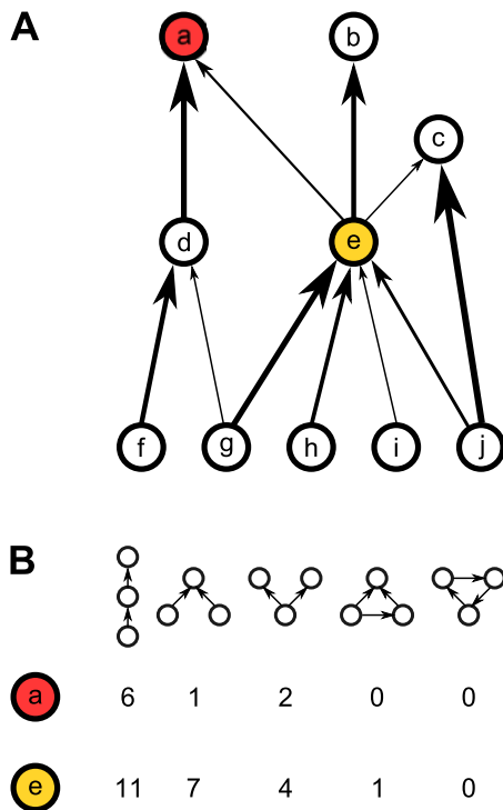
Fig. 2. Motif roles describe the way in which each species is embedded in a food web. They are defined by decomposing the web into its component motifs (unique configurations of n interacting species) and counting the number of times that each species appears in each motif. In A), we highlight two focal species. In B), we show the roles of these two species, defined based on three-species motifs. Note that while there are 13 different three-species motifs, this simple food web contains only one-way interactions and therefore is made up of the five motifs which contain one-way interactions exclusively. These five motifs are shown above the roles of species ‘a’ and ‘e’; note that the three-species loop motif does not occur in the roles of either species. Also note that each set of 3 interacting species represents only one motif: the motif which includes all interactions among those three species. For example, the set [c, e, j] represents the omnivory motif (second from right in the lower panel) but does not represent a three-species chain or direct competition motif (left and second from left) as these motifs do not capture all of the interactions within this set of species.
